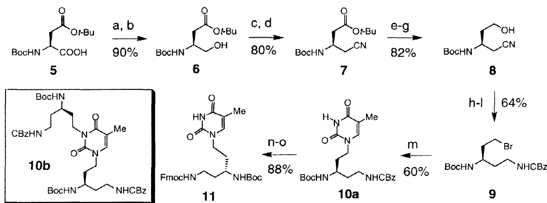
Scheme 1: (a) 1.1 eq iso -BuOCOC 2 Cl, NMM, THF, 0 °C; (b) 3 eq NaBH 4 , 0 °C MeOH; (c) TsCl, Pyr, rt; (d) 2.5 eq NaCN, DMSO, 80 °C; (e) 2M NaOH, MeOH, rt; (f) 1.1 eq iso -BuOCOC 2 Cl, NMM, DME, -15 °C; (g) 3 eq NaBH 4 , H 2 O, -15 °C; (h) TBDMSCl, imidazole, rt; (i) 0.4 eq CoCl 2 ·6H 2 O, MeOH, 10 eq NaBH 4 , -15 °C; (j) 10% K 2 CO 3 , Dioxane, 1.2 eq CBzCl; (k) 1.2 eq Bu 4 NF, THF, rt; (l) Ph 3 P, CBr 4 , THF, rt; (m) 3 eq Thymine, 3 eq K 2 CO 3 , Bu 4 NI (cat), DMF, 80 °C; (n) H 2 , 10% Pd/C, MeOH; (o) 1.2 eq FmocCl, 10% K 2 CO 3 , CH 3 CN.
